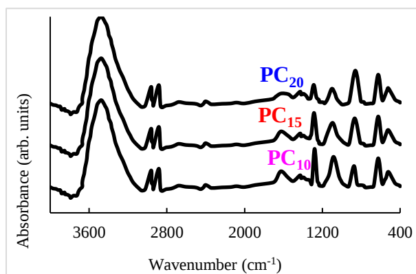
Fig. 4. FT-IR absorption spectra of P_2O_5 -CaO- Na_2O : CuO glasses.
